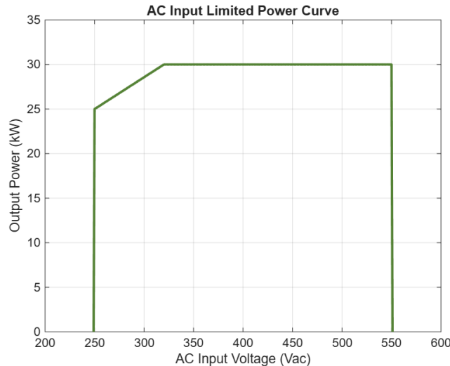
Figure 1-1 AC Input Power Limiting Curve
